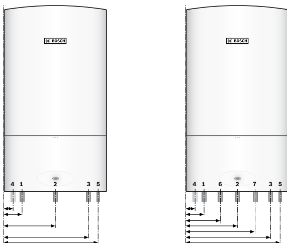
Figure 1 18kW & 30 kW ZSB models
