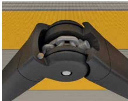
Folding arm technology Proven technology: single steel-link chain.
